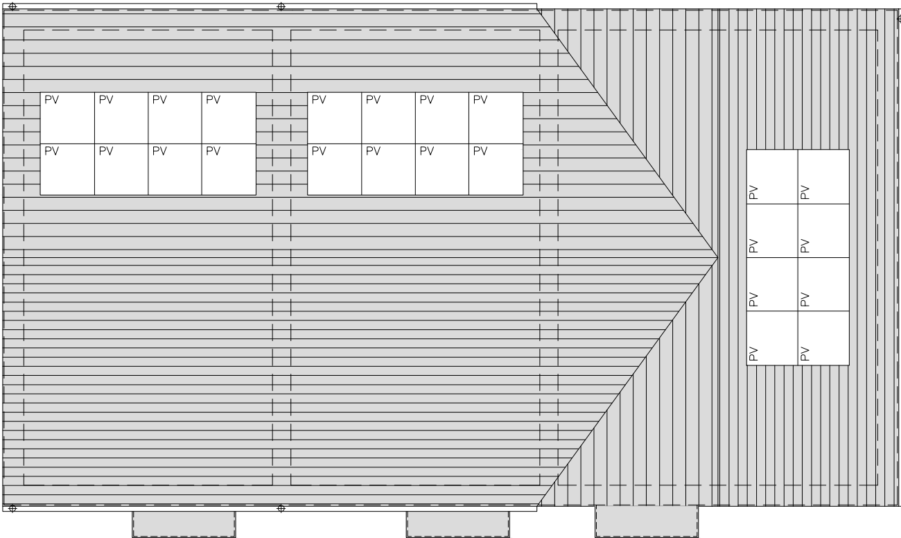
Roof Plan
